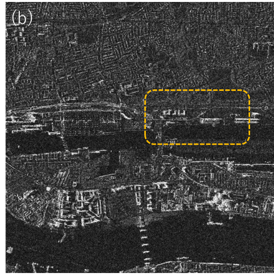
Figure 3.2 (a) 5m x 5m GRD image; (b) 1m x 1m SR-GRD image(Stripmap). The suppression of sidelobes is clearly noticeable for the bright target in the dashed rectangle.
